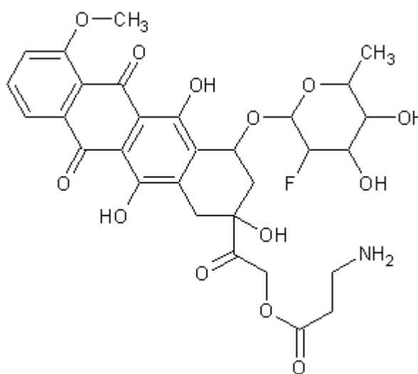
Molecular Structure:
